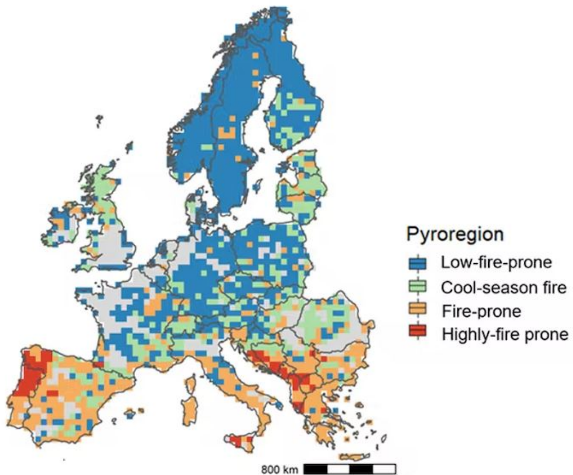
Distribution of 'pyro-regions' representing different fire characteristics across the continent.
