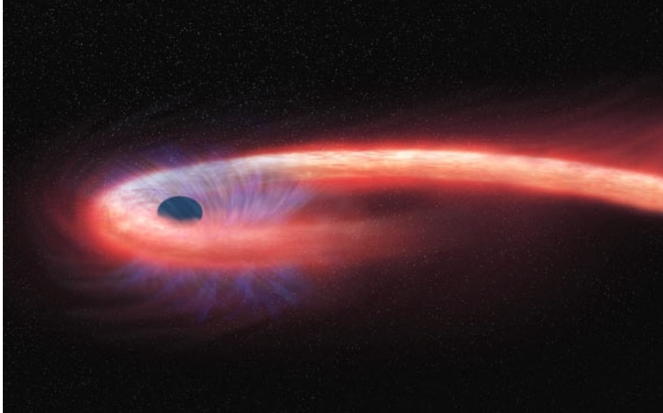
Tidal Disruption Event
